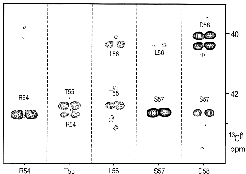
Figure 2. Regions of ( F_1, F_2 ) strips from the 600 MHz 3D [CO]HN(CA)CB-E.COSY spectrum of 3.5 mg ^{13}\text{C}/^{15}\text{N} -enriched ubiquitin (pH 4.7; 30 °C) in a 220 \mu\text{l} Shigemi microcell (1.8 mM) at 600 MHz, taken orthogonal to the F_3 ( ^1\text{H}^{\text{N}} ) axis at the ^1\text{H}^{\text{N}} and ^{15}\text{N} ( F_1 ) frequencies of Arg ^{54} -Asp ^{58} . The horizontal displacement for each doublet corresponds to ^1J_{\text{C}^{\text{N}}} , the small vertical displacement to ^3J_{\text{C}^{\text{C}}\beta} (intraresidue), or ^2J_{\text{C}^{\text{C}}\beta} for cases where ^{13}\text{C}_{i-1}^{\beta} is observed (strips of Thr ^{55} -Asp ^{58} ). The full ^{13}\text{C}^{\beta} spectral window is 10 ppm, and extensive aliasing occurs in this dimension.
