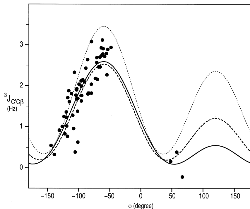
Figure 3. Relation between {}^3J_{C'C\beta} values measured with the [CO]HN(CA)CB-E.COSY experiment and protein backbone \phi angles in human ubiquitin. Lines correspond to the Karplus curve {}^3J_{C'C\beta} = A \cos^2(\phi - 120^\circ) + B \cos(\phi - 120^\circ) + C Hz. The thick solid line ( A = 1.28 ; B = -1.02 ; C = 0.30 ) represents the best fit between [CO]HN(CA)CB-E.COSY-derived {}^3J_{C'C\beta} values and \phi angles derived from the crystal structure. The values of the Karplus curve for \phi > 0^\circ are ill determined because of a lack of data points. The thick dashed line is the curve obtained with HN(CO)C-derived values (Hu and Bax, 1997) ( A = 1.61 ; B = -0.66 ; C = 0.26 ). The thin dashed line is the curve reported by Löhr et al. (1997) ( A = 2.54 ; B = -0.55 ; C = 0.37 ).
